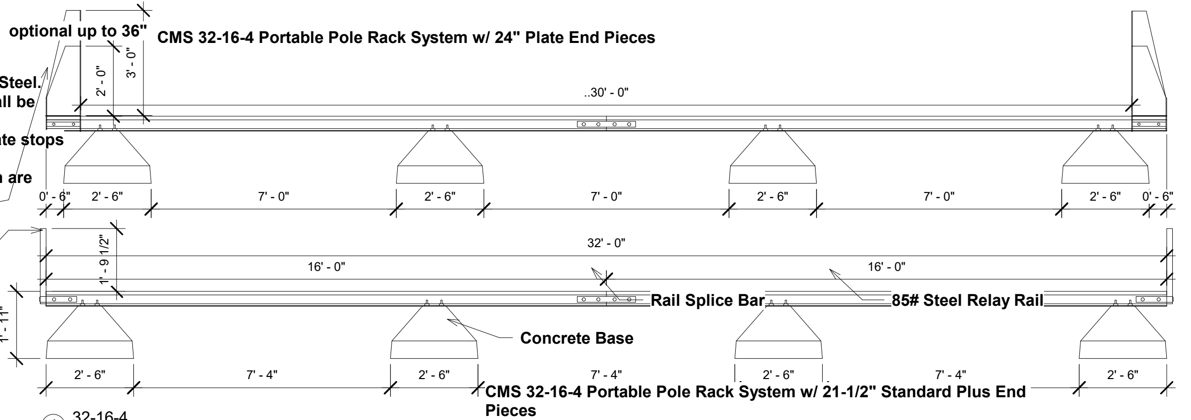
① 32-16-4 3/8" = 1'-0"
