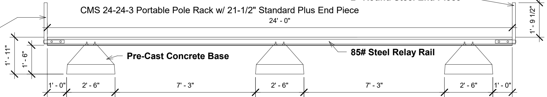
① 24-24-3 3/8" = 1'-0"
