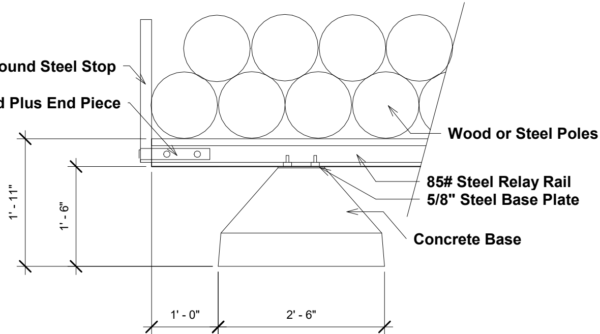
① 24-24-3 3/8" = 1'-0"
